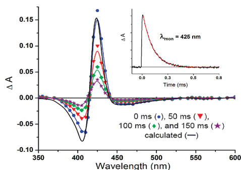
Figure 1. Absorption difference spectra ( \lambda_{ex} = 532 nm; 298 K) representing NO rebinding to [F_8Fe^{II}(\text{thf})_2] following photoejection from [F_8Fe^{II}(NO)(\text{thf})] ; the inset is a kinetic trace with a first-order fit.
