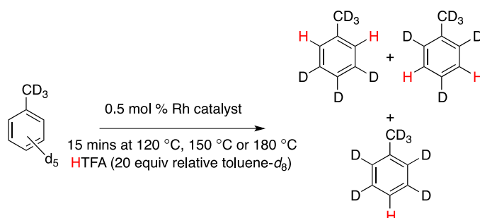
Scheme 5. Rhodium catalyzed H/D exchange between toluene- d_8 and HTFA.
