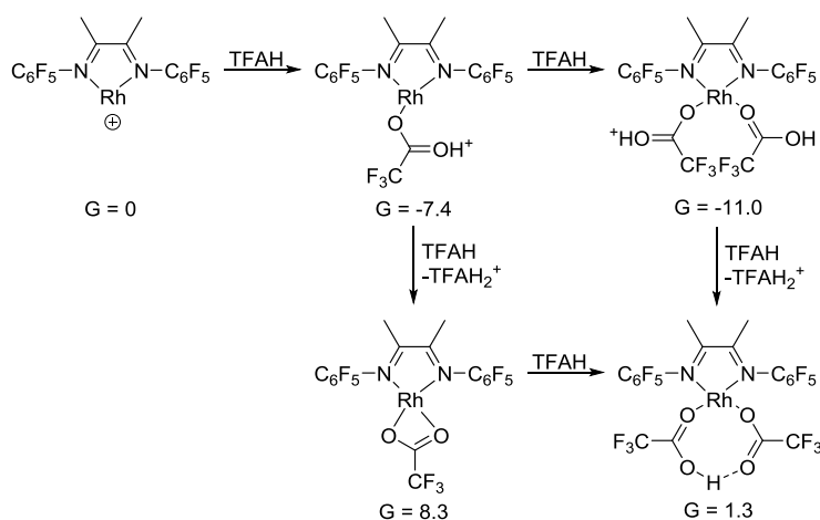
Scheme 7. Energetics of (11)\text{Rh}^+ complexing with TFAH. All free energies calculated at 150 °C and in kcal/mol. Note that the lowest energy species is (11)\text{Rh}(\text{TFAH})_2^+ (top right) and that release of a proton from this species to form (11)\text{Rh}(\text{TFAH})(\text{TFA}) (bottom right) is uphill by only 12.3 kcal/mol.
