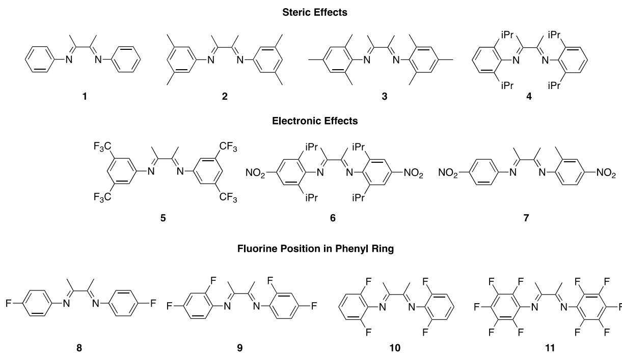
Scheme 2. Diimine proligands designed to vary the electron donor ability and steric profile of Rh I catalysts (iPr = isopropyl).
