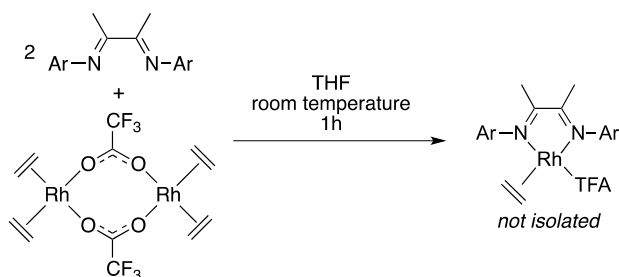
Scheme 3. General in situ synthesis of rhodium catalyst precursors from diimines and [Rh(\mu-TFA)(\eta^2-C_2H_4)_2]_2 .
