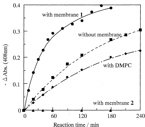
Figure 1. Electron injection rates from NADH to met-Mb via FMN in the presence of various matrix membranes. 5 \mu\text{M} Mb, 5 \mu\text{M} FMN, 1\text{mM} membrane, 250 \mu\text{M} NADH, in 10\text{mM} phosphate buffer ( \text{pH} = 7.0 ) at 38^\circ\text{C} . Reaction was monitored by the disappearance of 408\text{-nm} band.
