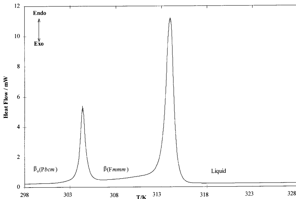
Figure 1. DSC curve of C_{21} with increasing temperature: observation of the o-d transition \beta(Pbcm) \rightarrow \beta(Fmmm) (first peak) and of the melting (second peak).
