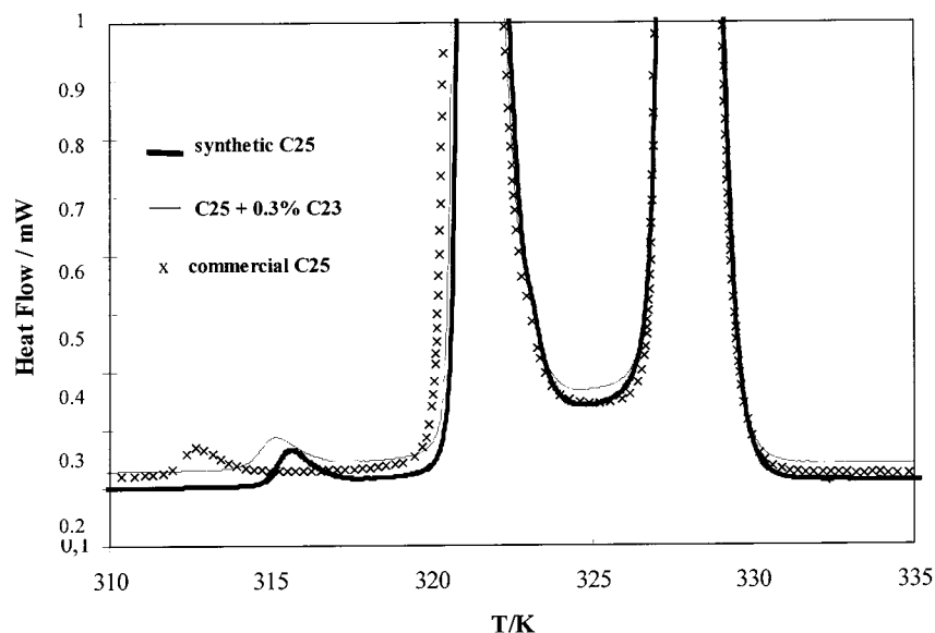
Figure 3. Influence of the impurities in the pure C 25 on the \delta -transition (first peak) and o-d transition (second peak) temperatures: the sample obtained by synthesis presents the higher solid–solid transition temperatures; when 0.3 molar % of C 23 is added to the C 25 synthetic sample, these transition temperatures decrease, but they are higher than those of the commercial C 25 . The \gamma -transition is not detected in the samples of high purity.
