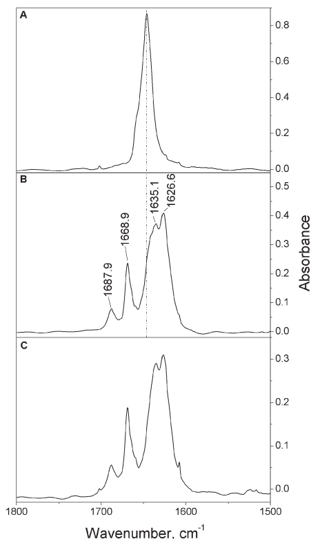
Figure 3. Measured IR spectra of copper guanidinate 1 and its thermolysis products (x axis, 1500–1800 \text{cm}^{-1} ; y axis, absorbance). Spectrum A: 2 in solid argon (thermolysis oven at 260 ^{\circ}\text{C} ); see Supporting Information, Figure S3 for a complete IR spectrum. Spectrum B: results of a thermolysis of complex 1 at 260 ^{\circ}\text{C} ; see Supporting Information, Figure S2 for a complete IR spectrum. Spectrum C: 3 in solid argon (thermolysis oven at 260 ^{\circ}\text{C} ); residual amounts of 2 have been electronically eliminated; see Supporting Information, Figure S4 for a complete IR spectrum.
