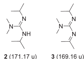
Chart 1. Protonated and Oxidized Ligand with Calculated Masses
