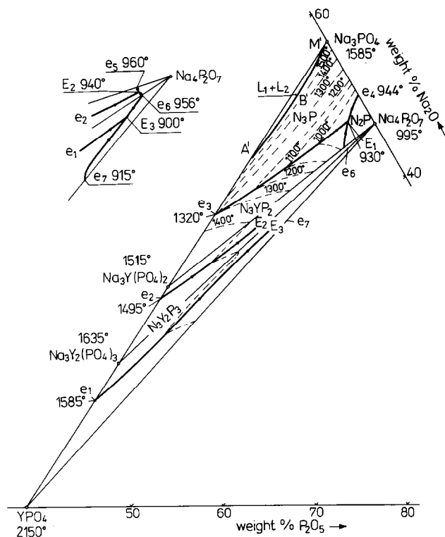
Fig. 4. Phase diagram of the system \text{YPO}_4\text{--Na}_3\text{PO}_4\text{--Na}_4\text{P}_2\text{O}_7 : \text{Na}_3\text{Y}_2\text{P}_3 = \text{Na}_3\text{Y}_2(\text{PO}_4)_3 ; \text{Na}_3\text{YP}_2 = \text{Na}_3\text{Y}(\text{PO}_4)_2 ; \text{Na}_3\text{P} = \text{Na}_3\text{PO}_4 ; \text{Na}_4\text{P}_2\text{O}_7 = \text{N}_2\text{P} .
