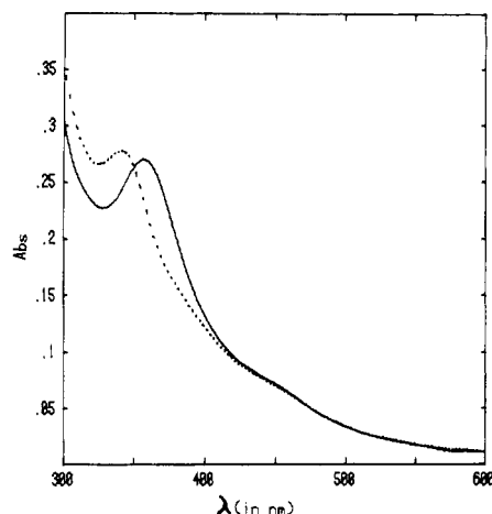
Figure 5. UV-vis spectrum of \text{H}_4\text{FeRu}_3(\text{CO})_{12} ( 7.7 \times 10^{-5} \text{ M} ) in methanol. Dashed curve results on addition of \text{NaOCH}_3 ( 5 \times 10^{-2} \text{ M} ).
