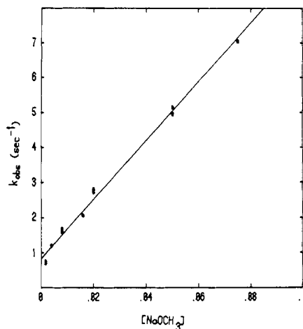
Figure 1. Kinetics plot of observed rate constants for the deprotonation of \text{H}_4\text{Ru}_4(\text{CO})_{11}(\text{P}(\text{OCH}_3)_3)_3 in methanol as a function of methoxide concentration.
