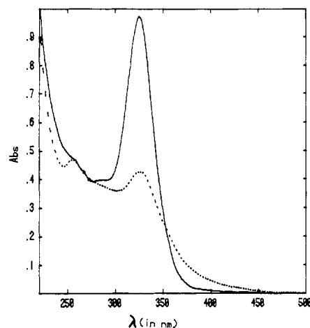
Figure 7. Electronic spectra of \text{H}_2\text{Os}_3(\text{CO})_{12} ( 3.5 \times 10^{-5} \text{ M} ) in methanol before (solid curve) and after (dashed curve) addition of sodium methoxide ( 5 \times 10^{-2} \text{ M} ).
