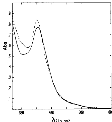
Figure 3. UV-visible spectrum of \text{H}_4\text{Ru}_4(\text{CO})_{11}(\text{P}(\text{OCH}_3)_3) ( 6 \times 10^{-5} M). Dashed curve results upon addition of sodium methoxide ( 5 \times 10^{-2} M).
