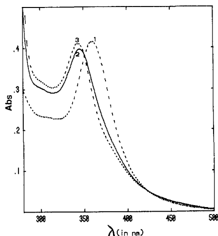
Figure 2. Electronic spectrum of \text{H}_4\text{Ru}_4(\text{CO})_{12} ( 2.5 \times 10^{-5} M) (1) in neutral methanol, (2) in pH 12.7 veronal/veronate buffered methanol, (3) in 2.5 \times 10^{-3} M \text{NaOCH}_3 in methanol.
