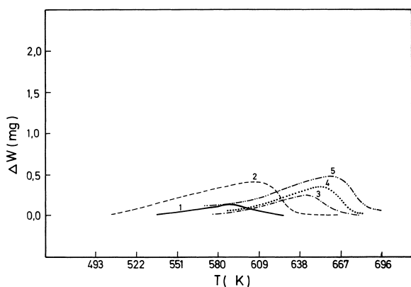
Fig. 4. TG diagrams of PbO under different \text{CO}_2 pressures. (1) 109; (2) 150; (3) 270; (4) 317; and (5) 371 torr.
