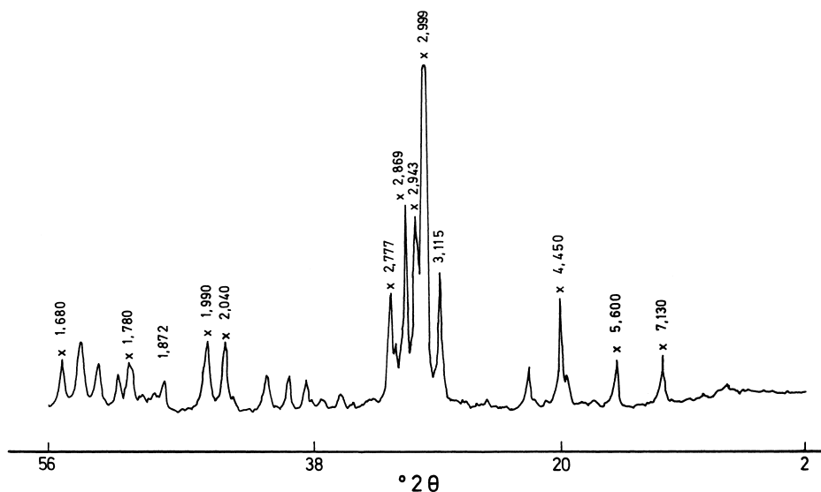
Fig. 5. XRD diagram of PbO carbonated at a \text{CO}_2 pressure of 150 torr at 320^\circ\text{C} . (X), \text{Pb}_3\text{O}_2\text{CO}_3
