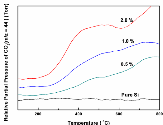
Figure 12. CO-TPR profiles of Mn-ZSM-5 (all silica, 0.5 %, 1 %, and 2 %).
