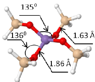
Figure 1. Model \text{Mn}(\text{OSiH}_2)_4^- compound with optimized geometric parameters. The atoms are colored with respect to atom type with Mn as violet, oxygen as red, silicon as light brown, and hydrogen as white.
