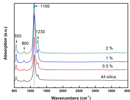
Figure 7. FT-IR spectra of Mn-ZSM-5 (all silica, 0.5 %, 1 %, and 2 %).
