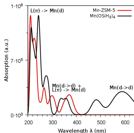
Figure 15. Simulated UV-Vis spectra of the model Mn(OSiH_3)_4^- compound and an Mn ion inserted into the zeolite framework.
