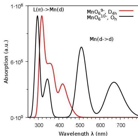
Figure 16. Simulated UV-Vis spectra of the six-coordinate \text{MnO}_6^{10-} , \text{Mn(II)} and \text{MnO}_6^{9-} , \text{Mn(III)} model oxides. For the \text{Mn}^{2+} ( d_5 ) oxide, an Mn-O distance of 2.00 Å with O_h symmetry was used, while the \text{Mn}^{3+} ( d_4 ) oxide was tetragonally distorted to D_{4h} symmetry, having distances of Mn-Oaxial = 2.20 Å and Mn-Oequatorial = 2.00 Å 48 .
