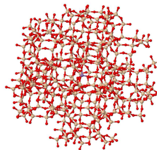
Figure 2. Embedded Mn-zeolite cluster \text{Mn}(\text{OSiH}_2)_4\text{Si}_{155}\text{O}_{591} . It is important to emphasize that terminal oxygen atoms were not capped which could have an influence on the overall structure of the cluster.
