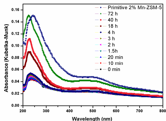
Figure 13. UV-Vis absorption spectra of degassed 2 % Mn-ZSM-5 after being exposed to air for different periods from 0~72 hours along with the absorption of the initial sample before degassing.
