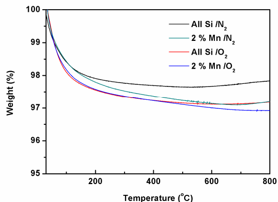
Figure 10. TGA analysis on Si-ZSM-5 and 2 % Mn-ZSM-5 under N 2 and O 2 atmospheres.
