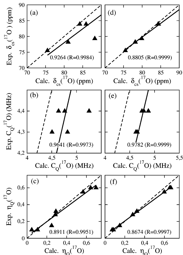
Figure 9. Comparison of experimental and calculated NMR parameters ( \delta_{\text{iso}} , C Q , η Q ) for (a, b, c) the published structures and (d, e, f) the DFT optimized structure of trimetaphosphate (Na 3 P 3 O 9 ) and tripolyphosphate (for Na 5 P 3 O 10 , sites O1, O2, only). For \delta_{\text{iso}} and C Q parameters, the graphs are restricted to the range of the nonbridging oxygens. The exact correlation between experimental and calculated values is represented by a dashed line. The slope of the linear regression is given with corresponding regression coefficients ( R ).
