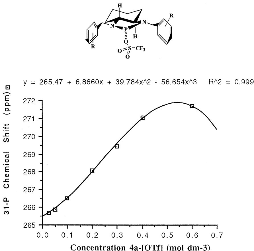
Fig. 9. Relationship between \delta_{\text{P}} (ppm) and concentration (mol dm ^{-3} ) for compound 4 ( \text{CH}_2\text{Cl}_2 ; 300 K).
