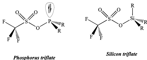
Fig. 4. Isoelectronic triflates.
