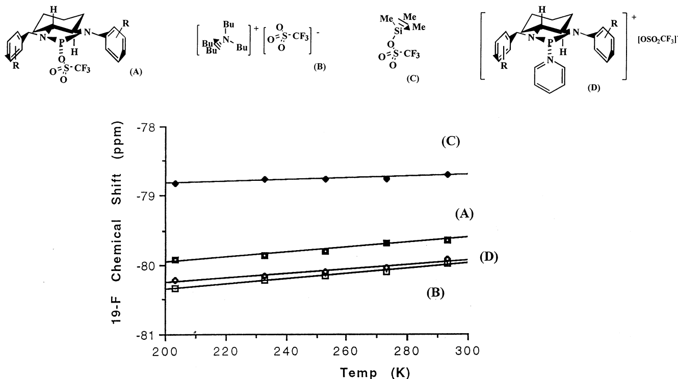
Fig. 11. Relationship between ^{19}\text{F} -NMR chemical shifts of 4 (■); 4-Py (◇); [\text{nBu}_4]^+[\text{OTf}]^- (○) and TMSOTf (◆) as a function of temperature ( \text{CH}_2\text{Cl}_2 ; 0.1 \text{ mol dm}^{-3} ).
