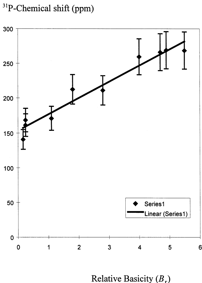
Fig. 13. Relationship between \delta_p (ppm) and relative basicity ( B_r ). Y-axis deviation bars are set at \pm 10\% .
