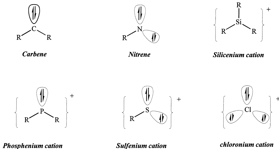
Fig. 3. Isoelectronic and isolobal relationship between main-group species.
