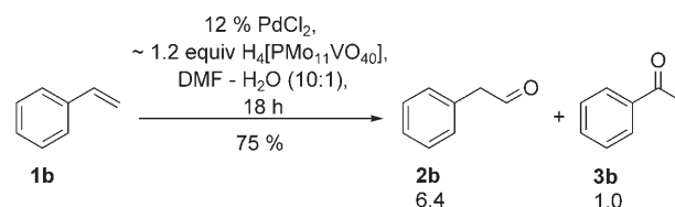
Scheme 8. Reoxidation of 1b using HPA.
