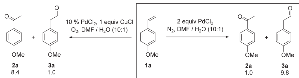
Scheme 2. Stoichiometric versus catalytic reaction.
