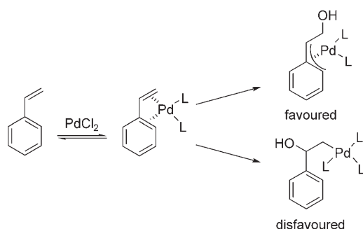
Scheme 6. Mechanistic proposal for the reversal of regioselectivity.
