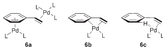
Scheme 4. Possible palladium–aryl interactions: 6a : face-on; 6b : \eta^4 -type; 6c : agostic (L = DMF, Cl, H 2 O).
