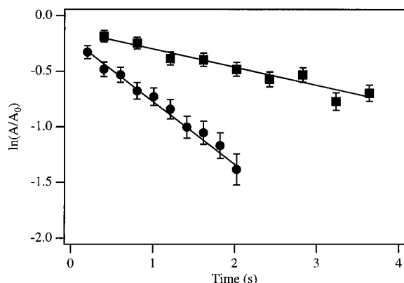
Figure 8. Plot of \ln(A/A_0) vs time for the reaction of \text{Ti}(\text{NMe}_2)_4 with \text{ND}_3 using He buffer gas. The \text{ND}_3 pressures are 0.0915 (■) and 0.364 (●) Torr.
