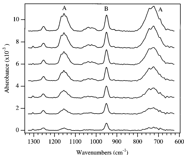
Figure 9. IR spectra of the reaction of \text{Ti}(\text{NMe}_2)_4 with \text{NH}_3 as a function of added \text{HNMe}_2 . The \text{NH}_3 was held constant at 0.46 Torr and the \text{HNMe}_2 pressure was varied from 0 (bottom) to 0.298 (top) Torr. Features are marked with A for \text{HNMe}_2 and B for \text{Ti}(\text{NMe}_2)_4 . Each spectrum is offset by 1.5 \times 10^{-3} absorbance units.
