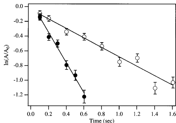
Figure 10. Effect of \text{HNMe}_2 on the reaction rate of \text{Ti}(\text{NMe}_2)_4 with \text{NH}_3 . The slope is k_{\text{obs}} and the open points have added \text{HNMe}_2 (0.198) and the solid points do not.
