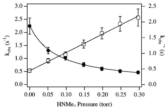
Figure 11. The dependence of k_{\text{obs}} (●) and (k_{\text{obs}})^{-1} (□) on \text{HNMe}_2 pressure. The \text{NH}_3 pressure was held constant at 0.46 Torr.
