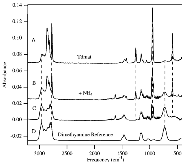
Figure 4. IR spectra of the reaction of \text{Ti}(\text{NMe}_2)_4 with \text{NH}_3 in the static cell: (A) initial spectrum of \text{Ti}(\text{NMe}_2)_4 alone, (B) \sim 7 s after addition of \text{NH}_3 , (C) after complete reaction, and (D) reference spectrum for \text{HNMe}_2 . The dashed lines indicate major features of \text{Ti}(\text{NMe}_2)_4 and \text{HNMe}_2 .
