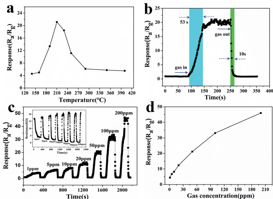
Fig. 8 (a) Sensitivity of the porous \text{ZnSnO}_3 nanocube sensor to 50 ppm formaldehyde under different test temperatures; (b) response–recovery curve of the porous \text{ZnSnO}_3 nanocube sensor to 50 ppm formaldehyde at 210 °C; (c) typical dynamic response–recovery curve of the porous \text{ZnSnO}_3 nanocube sensor to 1–200 ppm formaldehyde. The inset shows the curve of the sensor resistance to 1–200 ppm formaldehyde; (d) the response value curve of the porous \text{ZnSnO}_3 nanocube sensor to 1–200 ppm formaldehyde.
