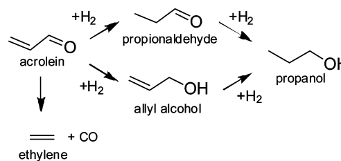
Scheme 1. Hydrogenation Pathways for Acrolein
