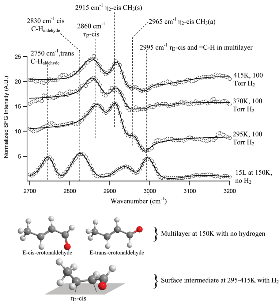
Figure 3. SFG-VS spectra of crotonaldehyde hydrogenation over Pt(111). The bottom spectrum was taken at 150 K after exposing the crystal to 15 L of crotonaldehyde to form a multilayer. The top three spectra were taken with 1 Torr of crotonaldehyde and 100 Torr of hydrogen over the Pt(111) crystal at the temperatures listed.
