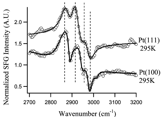
Figure 8. SFG-VS spectra of 1 Torr of crotonaldehyde and 100 Torr of hydrogen at 295 K over Pt(100) (bottom) and Pt(111) (top). SFG-VS spectra over Pt(111) and Pt(100) showed identical features at all temperatures from 295 to 415 K.
