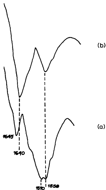
Fig. 1. \nu(\text{C}=\text{O}) region of IR spectra of the system \text{AlCl}_3/2,3,5,6\text{-tetramethyl-1,4-benzoquinone} at 2/1 (a) and 1/1 (b) mol ratios.
