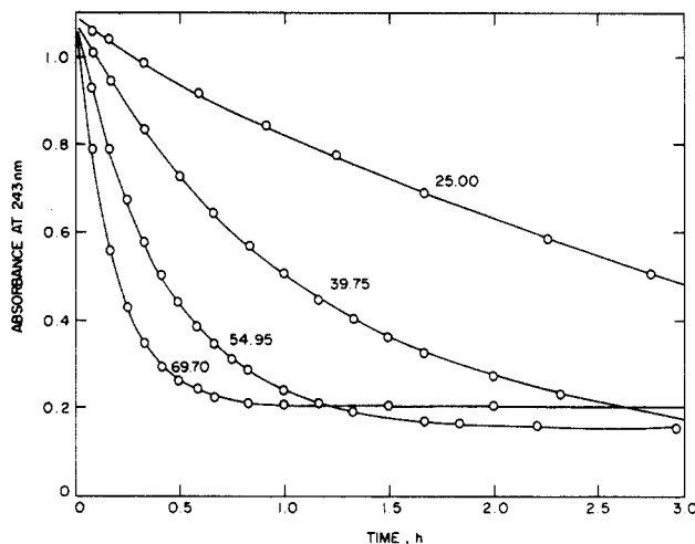
Figure 3. Effect of temperature on reaction of mesityl oxide in 17.25% \text{H}_3\text{PO}_4 (numbers on curves denote temperature in degrees Celsius).
