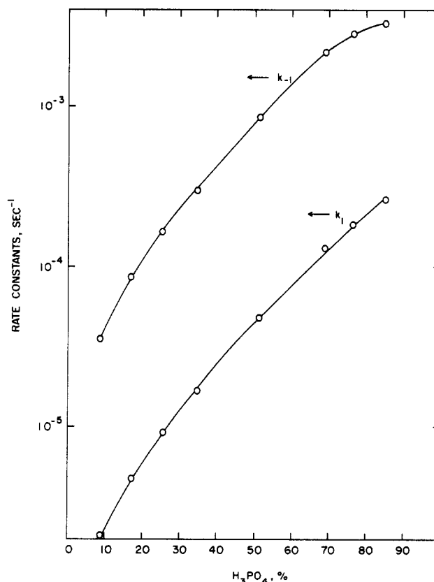
Figure 4. Effect of \text{H}_3\text{PO}_4 concentration on rate constants and in the system \text{H}_2\text{O} – \text{H}_3\text{PO}_4 –mesityl oxide–diacetone alcohol at 25 °C (organic concentration < 0.1\text{ m} ).
