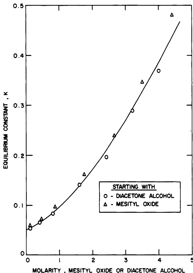
Figure 6. Effect of initial concentration of organic compounds on equilibrium constants at 25\text{ }^\circ\text{C} .
