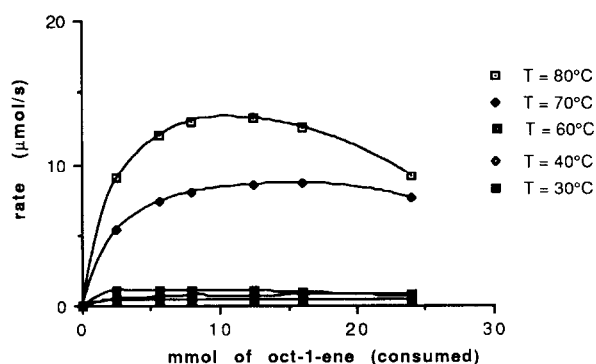
Fig. 1. Kinetic curves for the hydroformylation of oct-1-ene at 0.5 MPa of total pressure ( \text{H}_2/\text{CO} = 1/1 ) at various temperatures; [\text{Rh}_2(\mu\text{-S}^i\text{Bu})_2(\text{CO})_2(\text{PPh}_3)_2] = 1.05 \times 10^{-4} mol.
