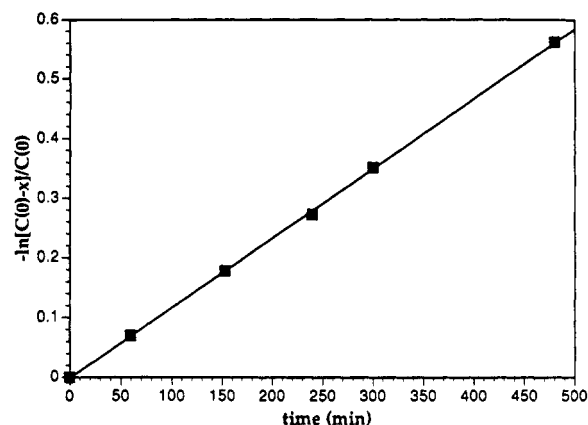
Figure 1. Kinetics of the coupling between iodobenzene and vinyltri- n -butyltin in the presence of \text{Pd}_2\text{dba}_3 and (pentafluorophenyl)diphenylphosphine in THF at 50 °C; 0.16 M each PhI and stannane, 3.2 mM Pd, and 12.8 mM phosphine. C(0) = 0.16 M, x = extent of conversion to styrene. Observed first-order rate constant: 1.12 \times 10^{-3} \text{ min}^{-1} .
