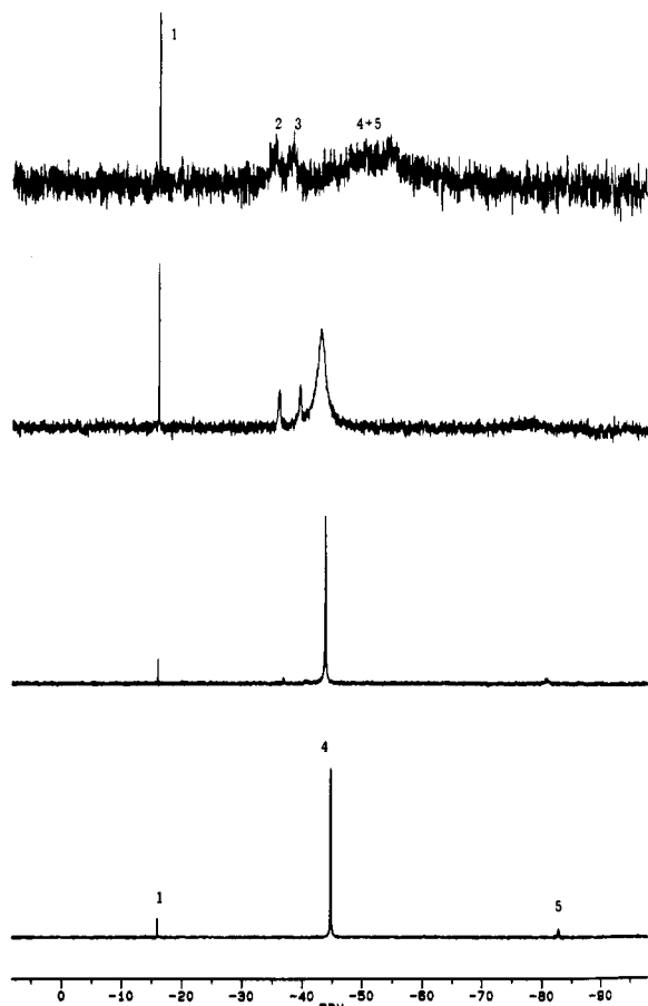
Figure 3. Low-temperature ^{31}\text{P} NMR study of \text{Pd(0)} -TFP complexes: ca. 13 mM \text{Pd}_2\text{dba}_3 in THF with 4 equiv of TFP per Pd. 1 = TFP oxide; 2,3 = mixed \text{Pd/dba/TFP} complexes; 4 = \text{Pd(TFP)}_4 ; 5 = TFP. Temperature: (a) 24 °C; (b) -23 °C; (c) -43 °C; (d) -60 °C.
