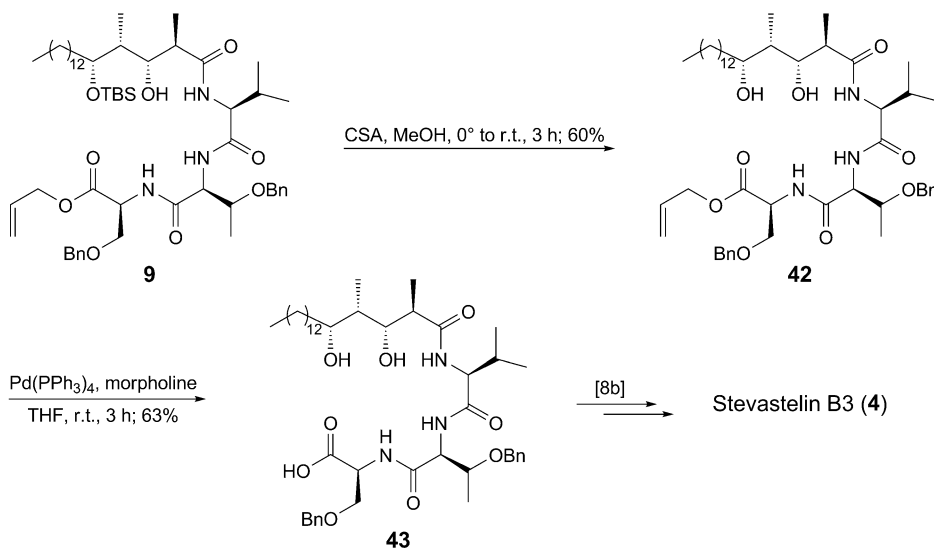
Scheme 10. Synthesis of the Key Precursor Diol 43
