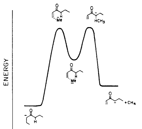
Figure 2. Mechanism proposed for the methane elimination g \rightarrow h . Using Benson's additivity rules 20 and an electron affinity (EA) of \text{C}_3\text{H}_7\text{COCHC}_2\text{H}_5 = 1.72 \text{ eV}^{21} and assuming an EA of 2.06 \text{ eV} for \text{CH}_2=\text{CHCOCHC}_2\text{H}_5 (by analogy with \text{EA}(\text{C}_6\text{H}_5\text{COCH}_2) = 2.06 \text{ eV}^{21} ), \Delta H_f for the overall process = +30 \text{ kJ mol}^{-1} .
