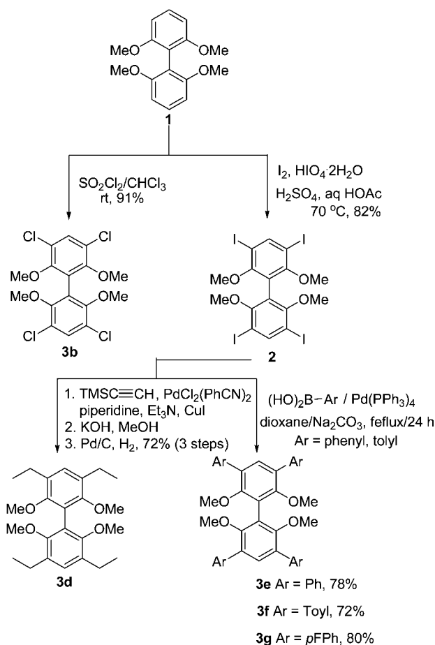
Scheme 2. Synthesis of 3,3',5,5'-Tetrasubstituted Biphenyl
