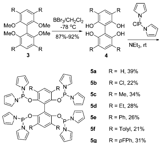
Scheme 3. Synthesis of Ligands
