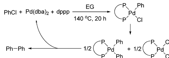
Scheme 7. Catalytic Homocoupling of ArCl in EG
