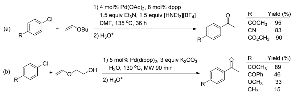
Scheme 5. Possible Effect of EG on the Formation of the Key Cationic Pd(II) Species
