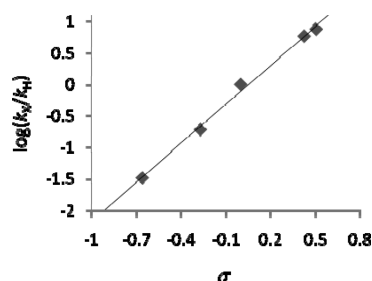
Figure 2. Plot of \log(k_X/k_H) vs Hammett substituent constant \sigma for the arylation of 2a with ArCl (see the Supporting Information for experimental details).
