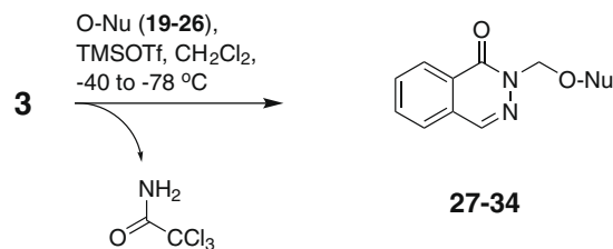
Scheme 2. The reaction of phthalazinone trichloroacetimidate with O-nucleophiles.
