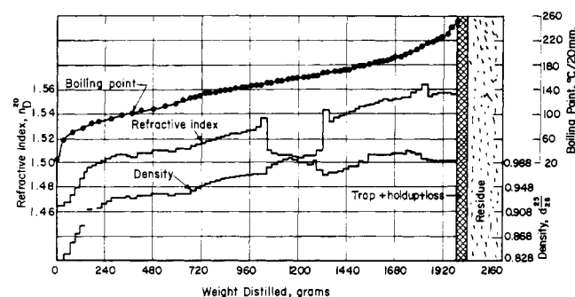
Figure 1. Fractionation by distillation of vacuum-flash distillate
