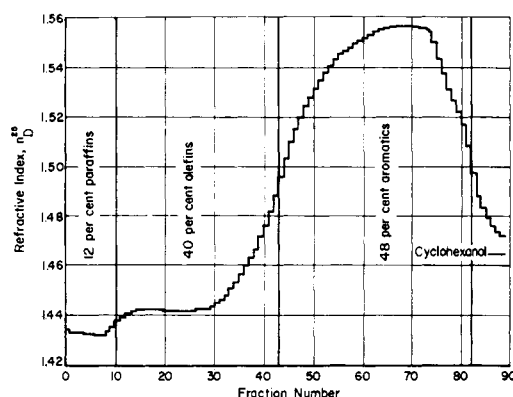
Figure 3. Silica gel adsorptogram for neutral oil
