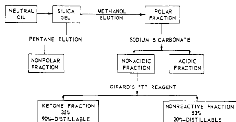
Figure 6. Study of polar compounds in neutral oil
