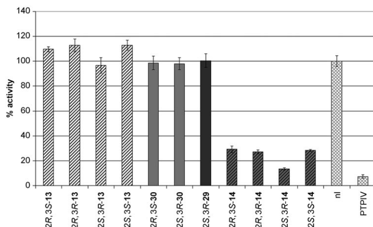
Figure 6. VHR inhibition at 100 µM inhibitor concentration. nI: control with no inhibitor; PTP inhibitor IV: control.
