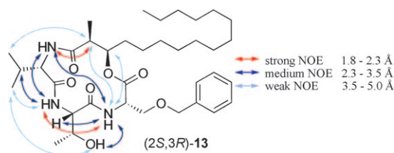
Figure 2. Selected ROESY contacts of macrocycle (2 S ,3 R )- 13 .
