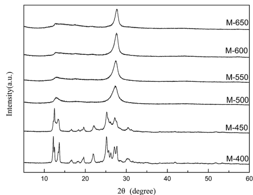
Fig. 1 XRD patterns of the M- x samples.
