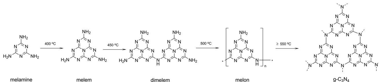
Fig. 3 Possible reaction pathway for the formation of melem and its derivatives by thermal condensation of melamine.
