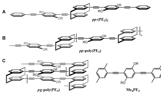
Figure 1. 1,4-Bis(phenylethynyl)-2,5-dialkoxybenzene ( \text{PE}_3 ) containing oligomers: (A) pseudo-para-[2.2]paracyclophane stacked dimer, pp\text{-(PE}_3)_2 ( R = n\text{-C}_{12}\text{H}_{25} , ref 4); (B) polymeric analog, pp\text{-poly(PE}_3) ( R = n\text{-C}_{12}\text{H}_{25} , ref 19); (C) pseudo-geminal polymer consisting of an extended stack, pg\text{-poly(PE}_3) , and unstacked \text{Me}_4\text{PE}_3 , R = n\text{-C}_9\text{H}_{19} .
