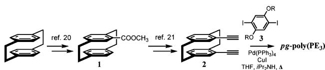
Figure 2. Preparation of pg\text{-poly(PE}_3) ( R = n\text{-C}_9\text{H}_{19} ).
