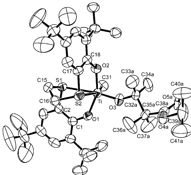
Figure 3. Molecular structure of the aldolate complex (edtpb)-TiMe(OCMe 2 CMe 2 CO 2 i Pr) ( 9 ) (hydrogen atoms were omitted for clarity, for the atoms of the ester alkoxy group only one the refined split positions are shown). Selected bond lengths (Å) and angles (deg): Ti–O1, 1.8815(16); Ti–O2, 1.8898(15); Ti–O3, 1.7622(16); Ti–S1, 2.7156(8); Ti–S2, 2.7227(8); Ti–C31, 2.099(2); Ti–O3–C(32a), 147.4(3); O3–Ti–C31, 102.43(9); O1–Ti–C31, 96.38(9); O2–Ti–C31, 95.45(8); O1–Ti–O2, 154.44(7); S1–Ti–S2 77.05(2).
