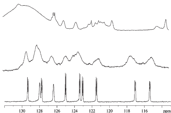
Figure 3. Gated decoupled ^{13}\text{C} NMR spectra in the aromatic/olefinic region of strychnine in \text{CDCl}_3 (bottom), in \text{CDCl}_3/\text{Poly-L-1} (middle) and in \text{CDCl}_3/\text{PBLG} (top).
