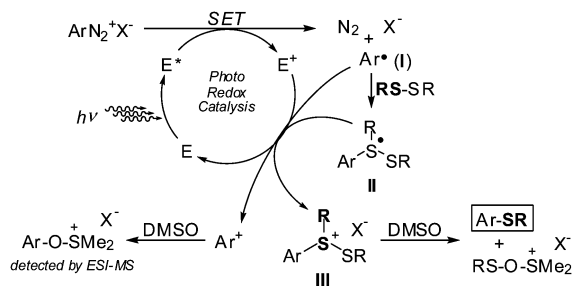
Scheme 4 Proposed reaction mechanism.
