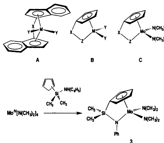
Scheme 1. Conditions: \text{Et}_2\text{O} , 12 h, 25°C, -2 \text{ HN}(\text{CH}_3)_2 .
