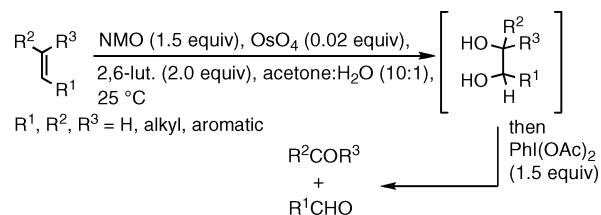
Scheme 5. Cleavage of Olefins to Aldehydes and/or Ketones by NMO, \text{OsO}_4 (cat.)/ \text{PhI}(\text{OAc})_2 in the Presence of 2,6-Lutidine
