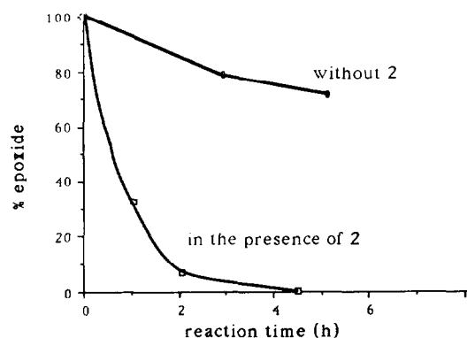
Fig. 1. Influence of the Bi catalyst 2 (5%) on the oxidation of styrene oxide ( 1a ) in DMSO at 80°C.
