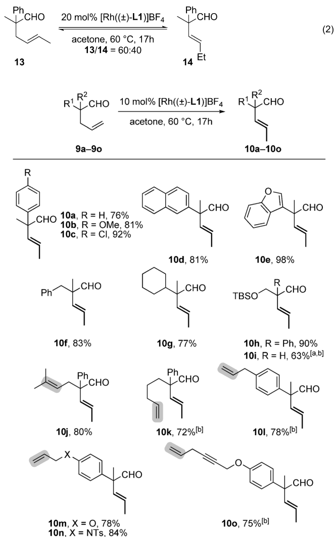
Scheme 2. Scope of the chemo- and stereoselective isomerization of 4-pentenals into ( E )-3-pentenals. All of the yields are given for isolated products as the average of two experiments; see the Supporting Information. [a] Yield determined by ^1\text{H} NMR spectroscopy in [\text{D}_6] acetone in the presence of an internal standard. [b] Room temperature. TBS = tert -butyldimethylsilyl. Ts = p -tolylsulfonyl.
