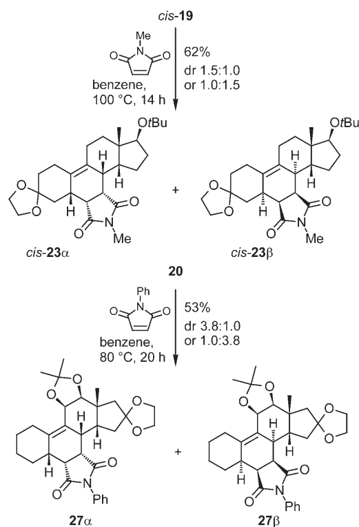
Scheme 6. Diels-Alder reactions of the tricyclic dienes cis -19 and 20 with N -methyl- and N -phenylmaleimide, respectively.
