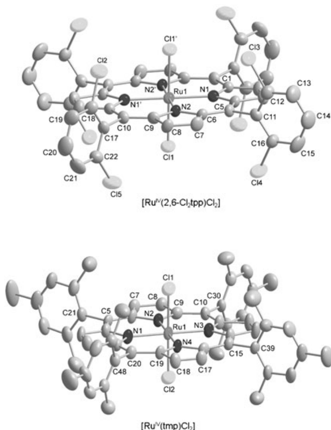
Figure 1. Structures of [\text{Ru}^{\text{IV}}(2,6\text{-Cl}_2\text{tp})\text{Cl}_2] and [\text{Ru}^{\text{IV}}(\text{tmp})\text{Cl}_2] with omission of hydrogen atoms. Thermal ellipsoids were drawn at a 30% probability level. Note that the unit cell of [\text{Ru}^{\text{IV}}(\text{tmp})\text{Cl}_2] contains two independent types of molecules, only one of which is shown here.
