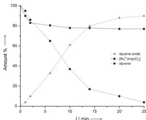
Figure 6. Time course plots for epoxidation of styrene with 2,6- \text{Cl}_2\text{pyNO} catalyzed by [\text{Ru}^{\text{IV}}(\text{tmp})\text{Cl}_2] (catalyst/styrene/2,6- \text{Cl}_2\text{pyNO} = 1:100:100). The reactions were monitored by ^1\text{H} NMR spectroscopy (300 MHz, \text{CDCl}_3 ) with 1,3,5-tribromobenzene as internal standard.
