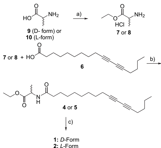
Scheme 1. Synthetic routes for amphiphiles 1 and 2 . (a) SOCl 2 , EtOH, 86%; (b) DCC, HOBT, EA, 95%; (c) NaOH, MeOH, H 2 O, 95%. DCC=1,3-dicyclohexylcarbodiimide, HOBT=1-hydroxybenzotriazole, EA=ethyl acetate.
