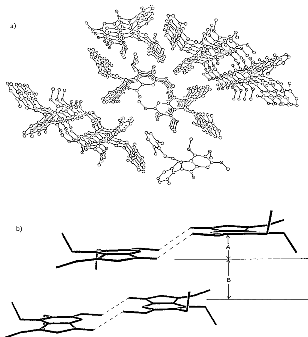
Figure 5. (a) Packing diagram along the a axis of compound 15 in the solid state. (b) Another perspective showing the hydrogen bond interactions and interplanar distances; A = 1.23 Å, B = 3.92 Å.
