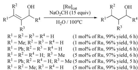
Scheme 3 Reduction of allylic alcohols using water as the solvent.
