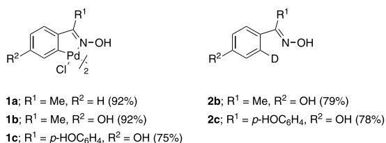
Fig. 1. Oxime-derived palladacycles and deuterated oximes.
