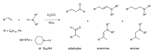
Scheme 1 Rhodium-catalyzed hydroaminovinylation of \alpha -olefins.
