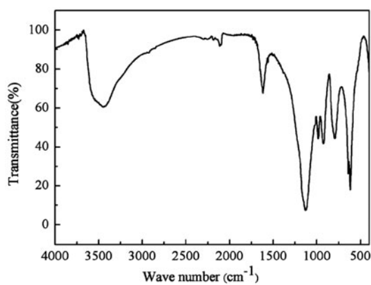
Figure 5. IR spectra of H 4 SiW 12 O 40 .
