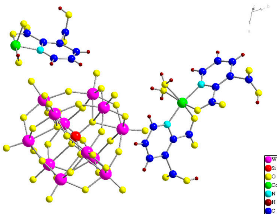
Figure 1. Crystal structure of the complex.
