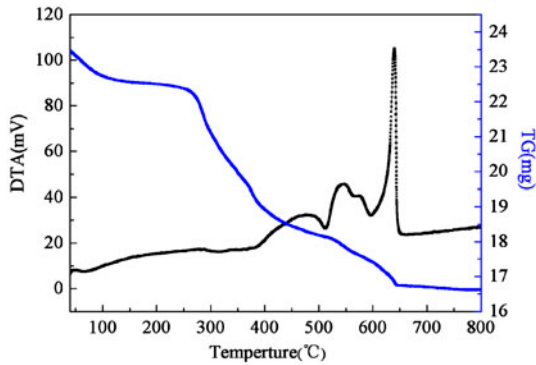
Figure 7. DTA and TG diagrams of the complex.
