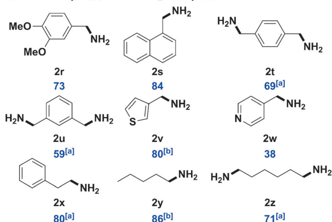
Scheme 3. Cobalt-catalyzed transfer hydrogenation of nitriles to primary amines. Reaction conditions: 1 (0.5 mmol), AB (0.8 mmol) in 1 mL of n -hexane, GC yield (%) were shown using biphenyl as the internal standard. [a] The reaction temperature was 100°C. [b] The reaction temperature was 120°C.
