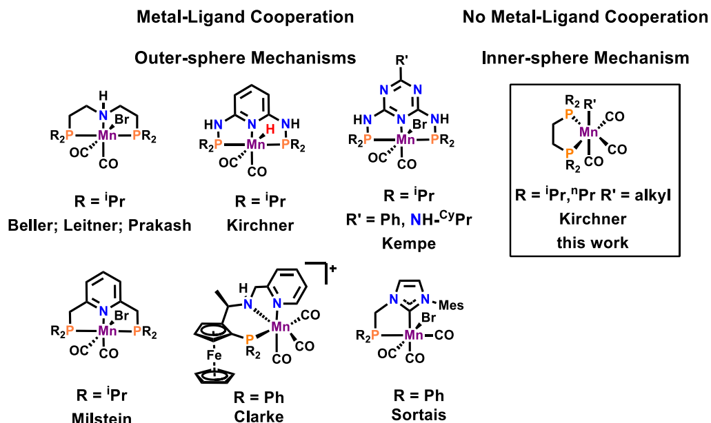
Scheme 1. Selected Mn(I) Precatalysts for Hydrogenation Reactions
