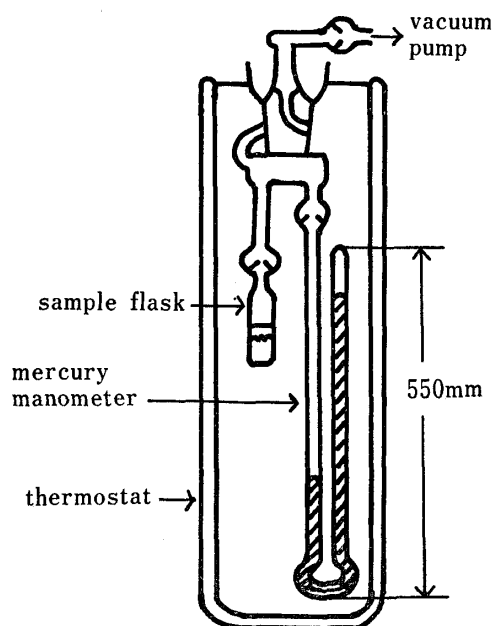
Fig. 2. Apparatus for Vapor Pressure Measurement
