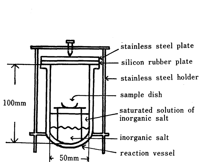
Fig. 1. Apparatus for Kinetics Study
