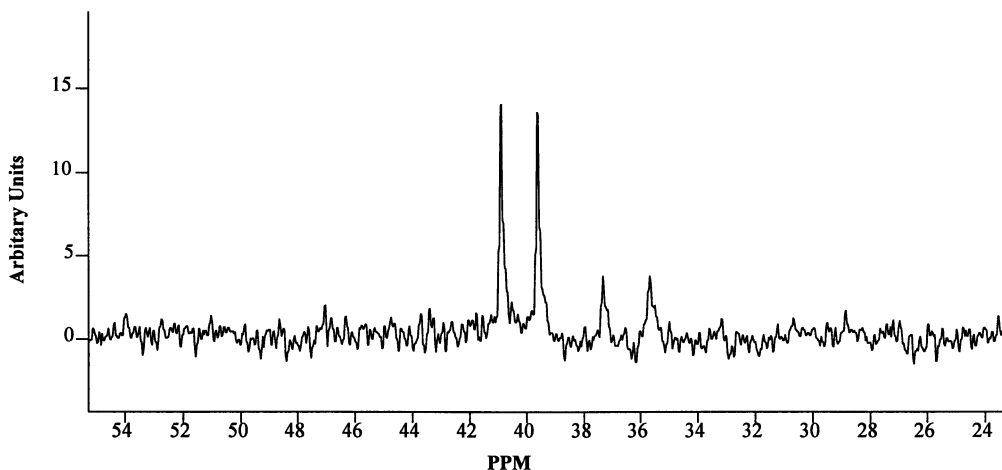
Fig. 5. ^{31}\text{P}\{^1\text{H}\} -NMR spectrum of a mixture containing \text{HRh}(\text{CO})((p\text{-CF}_3\text{C}_6\text{H}_4)_3\text{P})_2(\eta^2\text{-C}_2\text{H}_4) and \text{HRh}(\text{CO})((p\text{-CF}_3\text{C}_6\text{H}_4)_3\text{P})_3 in \text{CO}_2 at 0^\circ\text{C} and 207 bar. This spectrum was obtained after exposure of \text{HRh}(\text{CO})((p\text{-CF}_3\text{C}_6\text{H}_4)_3\text{P})_3 to \sim 10 bar of ethylene.
