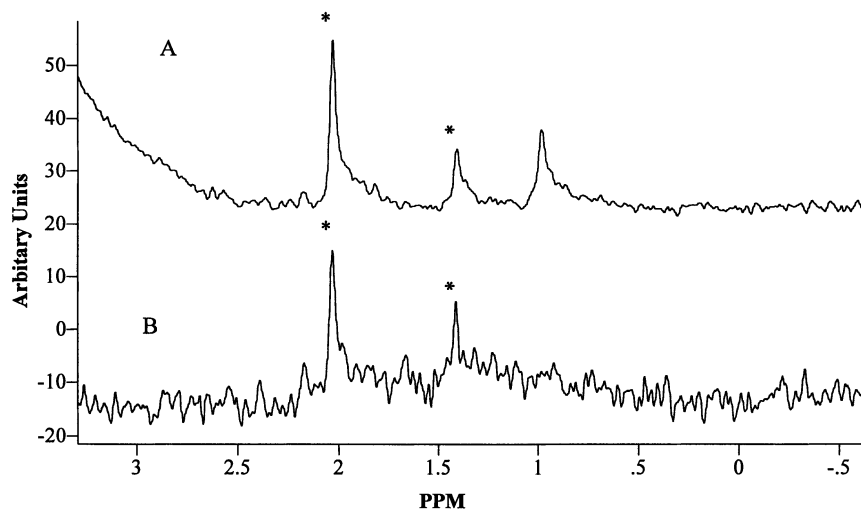
Fig. 4. (A) ^1\text{H} -NMR spectrum of \text{HRh}(\text{CO})((p\text{-CF}_3\text{C}_6\text{H}_4)_3\text{P})_3 and ethylene (12.5 bar) in \text{CO}_2 at 207 bar and 0^\circ\text{C} and (B) ^1\text{H} -NMR spectrum of \text{HRh}(\text{CO})((p\text{-CF}_3\text{C}_6\text{H}_4)_3\text{P})_3 in \text{CO}_2 at 207 bar and 0^\circ\text{C} , before exposure to ethylene. The peaks labeled by * are due to the enol form of acetylacetone from the Rh precursor molecule.
