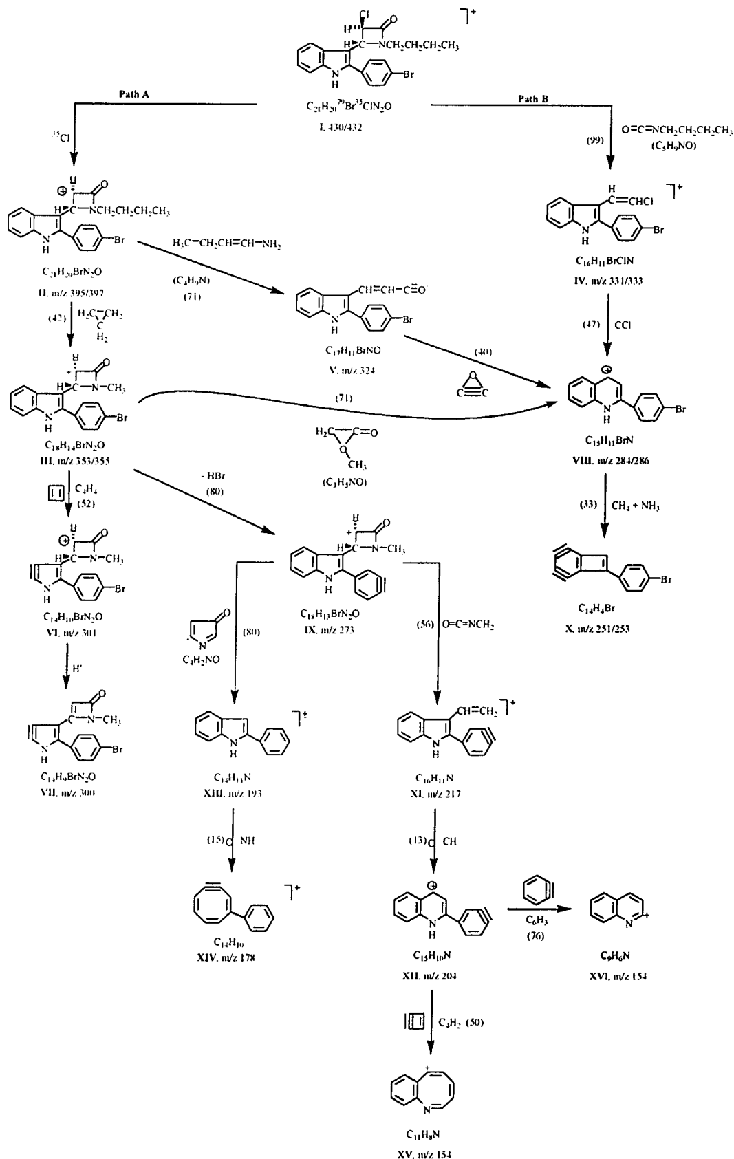
SCHEME 3 Mass fragmentation pattern of 1-butyl-3-chloro-4-[2-(4-bromophenyl)-1H-indol-3-yl]-2-azetidinone ( 4h ).
