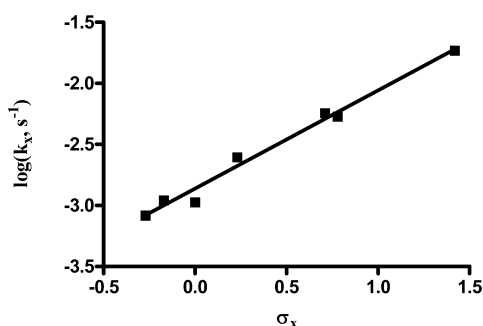
Figure 1. Hammett plot of \log(k_x) vs \sigma_x for the Cu(II)-promoted cleavage of 4a–g ( 5 \times 10^{-4} M) in methanol at 25 °C in the plateau region (7–8) of the \text{pH}/\log(k_x) profile. The line through the data is generated from a linear regression to provide \rho_x = 0.80 \pm 0.05 ; r^2 = 0.9844 (7 data).
