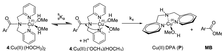
Scheme 1. Simplified Scheme for the \text{pH} Dependent Decomposition of 4 :Cu(II):( \text{OCH}_3 )( \text{HOCH}_3 ) to Form Cu(II): N,N -bis(2-picolyl)amine (Cu(II):DPA) and the Corresponding Methyl Benzoate (MB)
