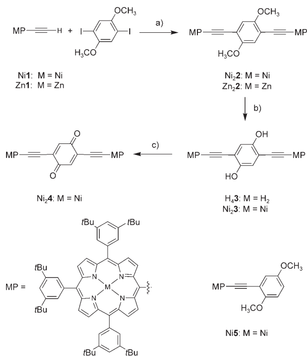
Scheme 1. Synthesis of porphyrin dimers. a) AsPh 3 , [Pd 2 (dba) 3 ], NEt 3 (Ni 2 2, 82%; Zn 2 2, 89%). b) i) Zn 2 2, 20% HCl, CH 2 Cl 2 ; ii) BBr 3 , CH 2 Cl 2 ; iii) Ni(OAc) 2 ·4H 2 O, CHCl 3 /AcOH (Ni 2 3, 43% over 3 steps); c) PbO 2 , CH 2 Cl 2 (90%).
